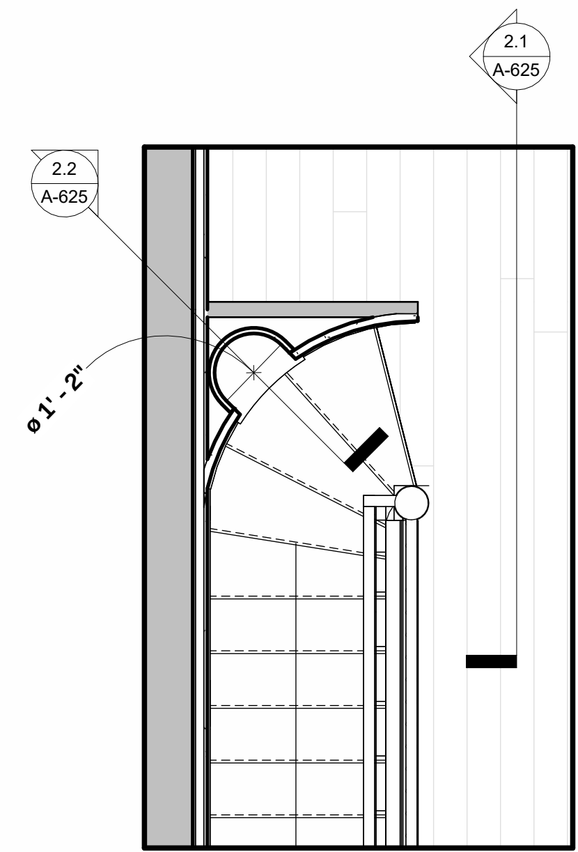
2 002 - UPPER STAIR LANDING PLAN 1/2" = 1'-0"
