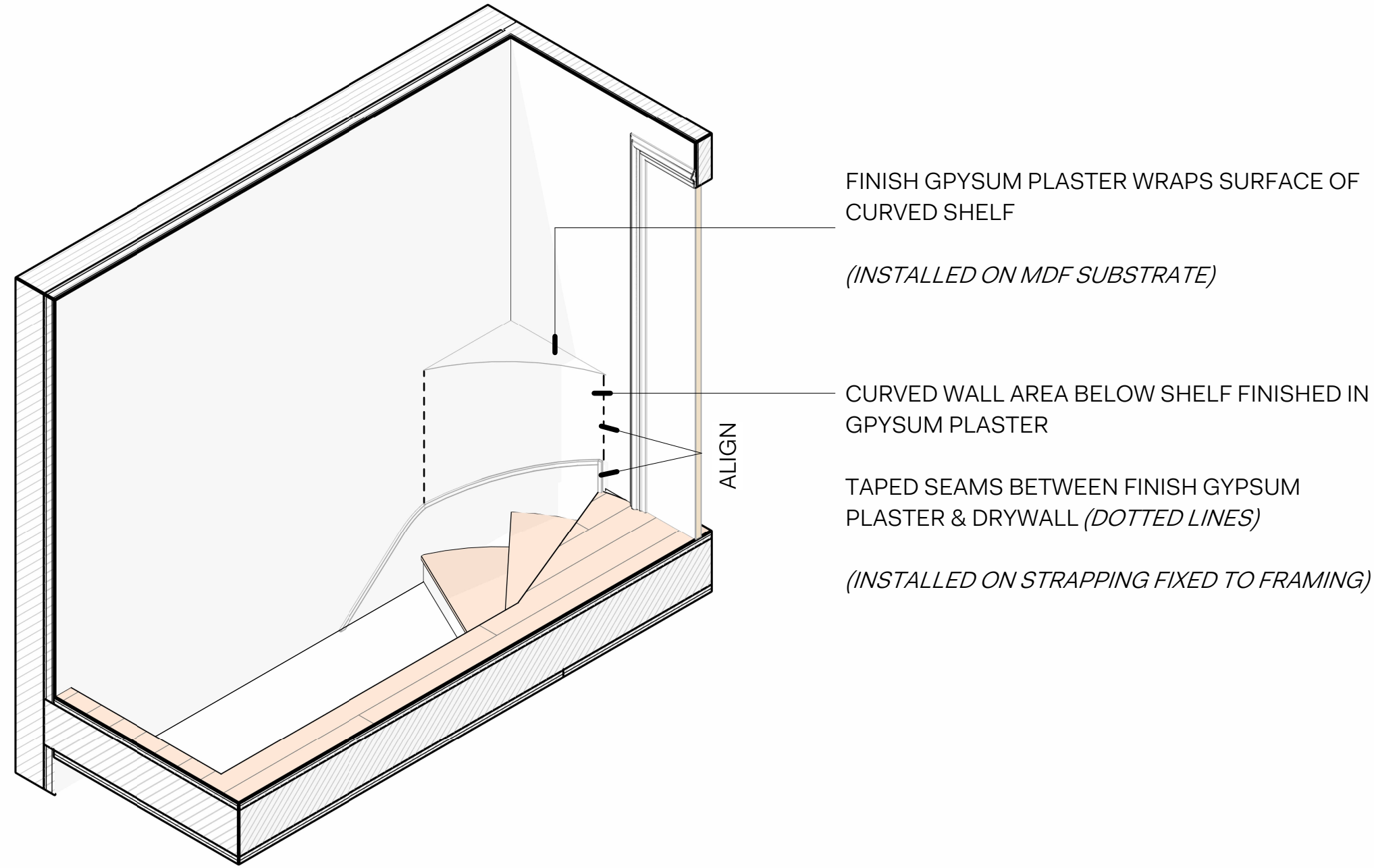
1 003 - UPPER STAIR LANDING CURVED SHELF & WALL PLASTER DETAIL
